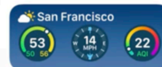
Configurable widgets
